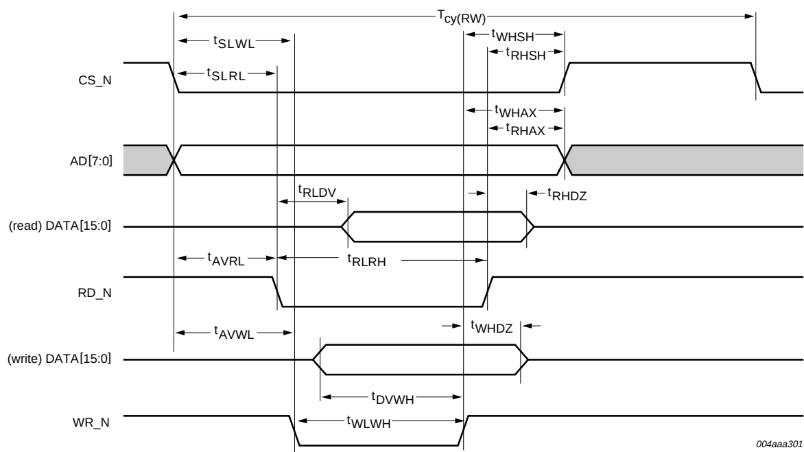
Fig 20. ISP1583 register access timing: separate address and data buses (8051 style).
