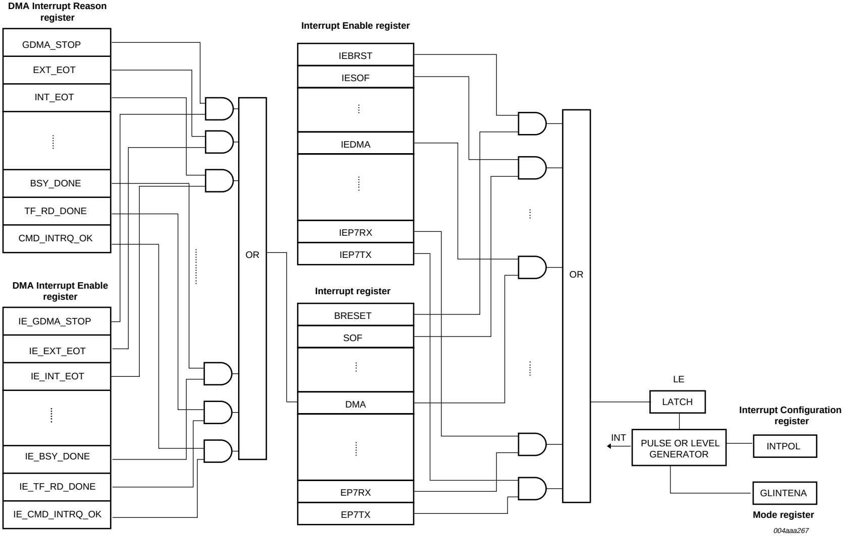
Fig 4. Interrupt logic.
