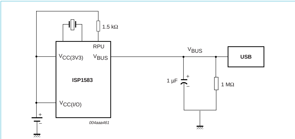
Fig 14. Self-powered mode.
