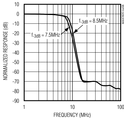
RECEIVER FILTER RESPONSE (1MHz TO 100MHz)
