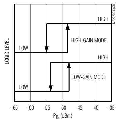
RECEIVER DETECTOR HYSTERESIS vs. INPUT POWER
