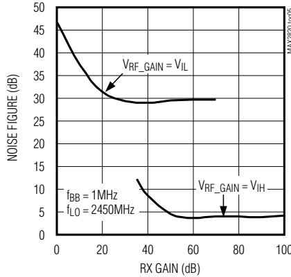
RECEIVER NOISE FIGURE vs. GAIN
