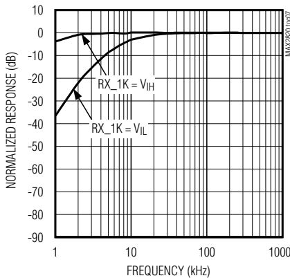
RECEIVER FILTER RESPONSE (1kHz TO 1MHz)
