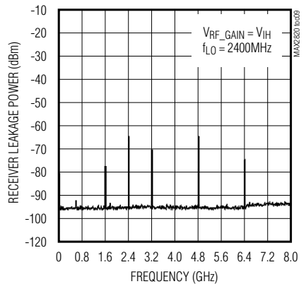
RECEIVER LEAKAGE SPECTRUM
