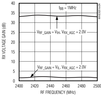
RECEIVER VOLTAGE GAIN vs. RF FREQUENCY
