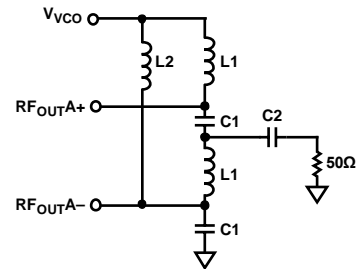
Figure 39. LC Balun for the ADF4351
