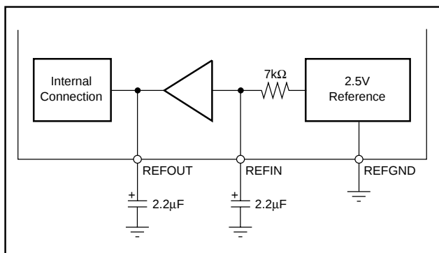
FIGURE 3. Reference Voltage Connection.
