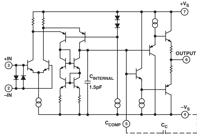
Figure 6. Simplified Schematic
