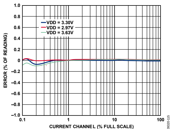
Figure 19. Current Channel B Active Energy Error as a Percentage of Reading (Gain = 1, Temperature = 25°C, Power Factor = 1) over Supply Voltage with Internal Reference, Integrator Off
