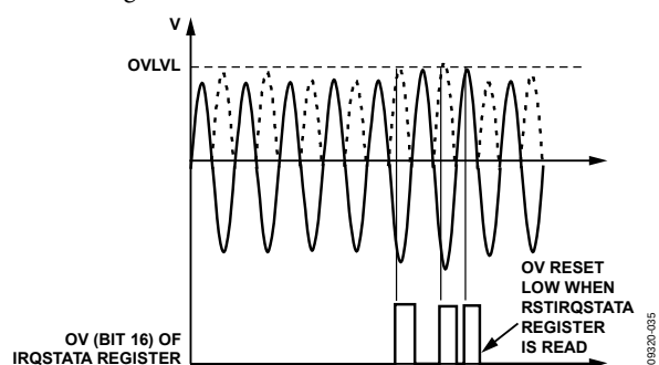
Figure 66. Overvoltage Detection
