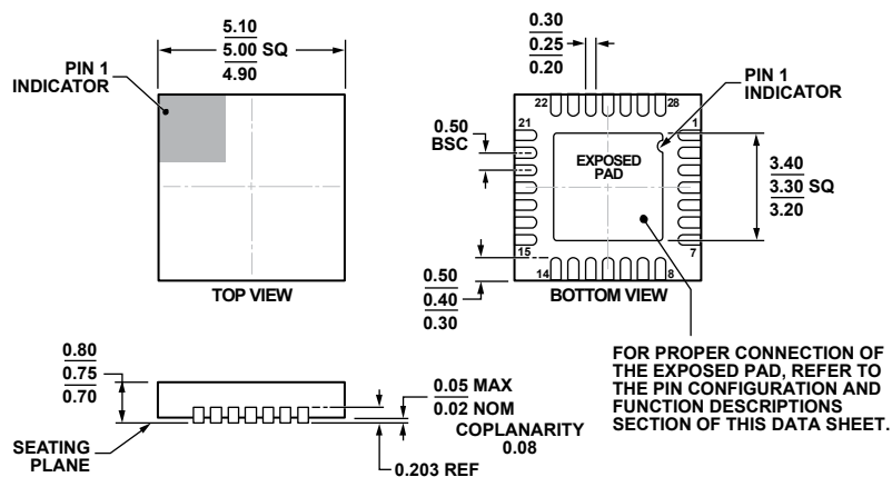
Figure 77. 28-Lead Lead Frame Chip Scale Package [LFCSP_WQ] 5 mm × 5 mm Body, Very Very Thin Quad (CP-28-6)
