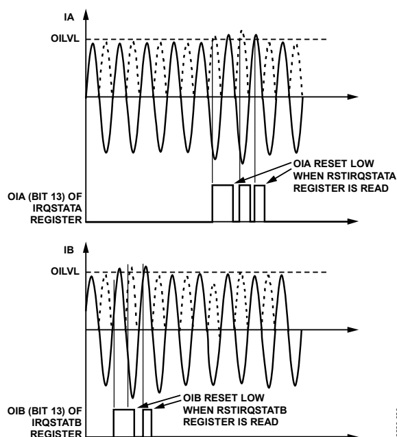
Figure 67. Overcurrent Detection
