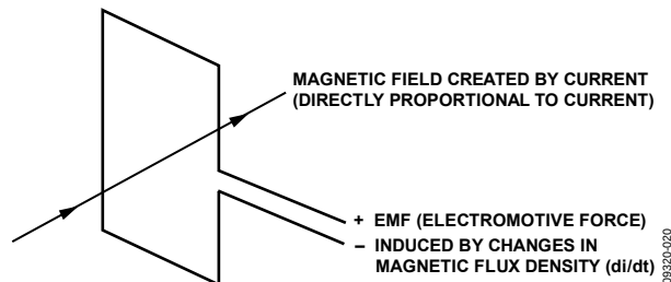
Figure 40. Principle of a di/dt Current Sensor
