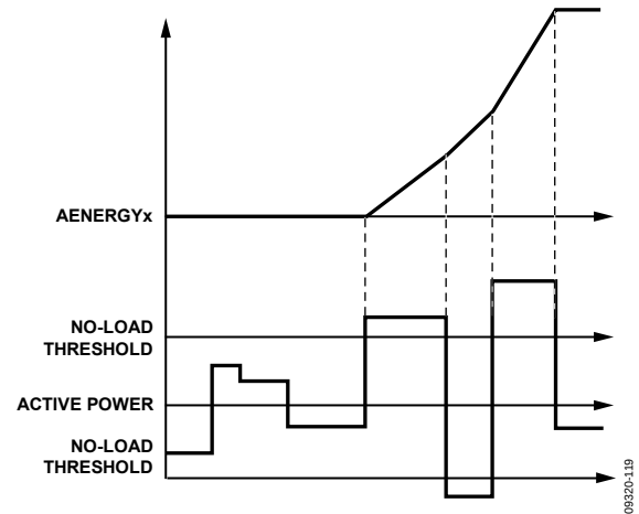
Figure 50. Active Energy Absolute Accumulation Mode
