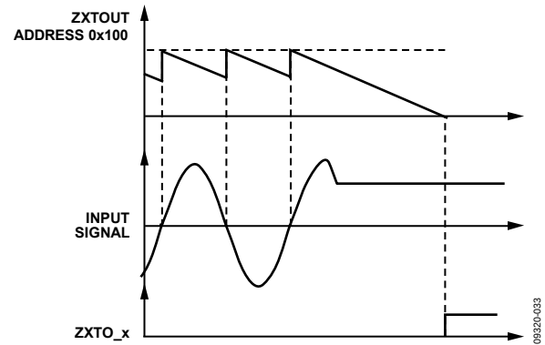
Figure 64. Zero-Crossing Timeout
