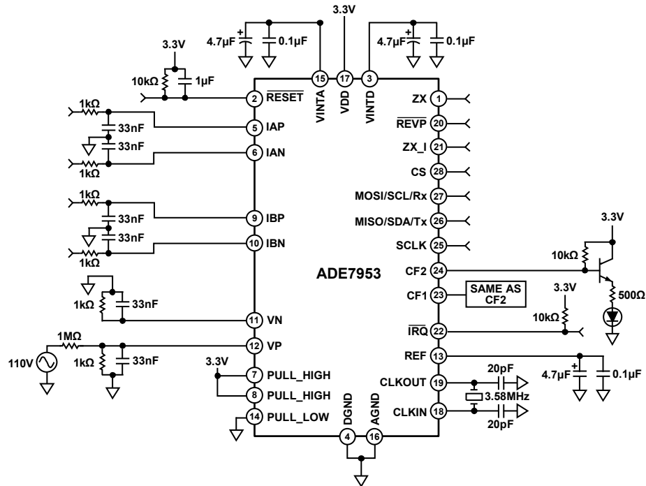
Figure 35. Test Circuit
