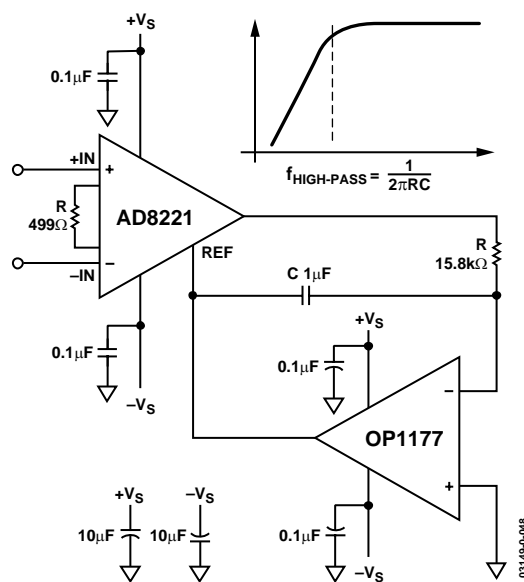
Figure 52. AC-Coupled Circuit
