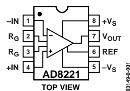
Figure 43. Pinout Diagram
