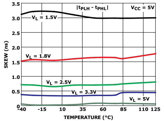
FIGURE 18. ISL3217XE RECEIVER SKEW vs TEMPERATURE
