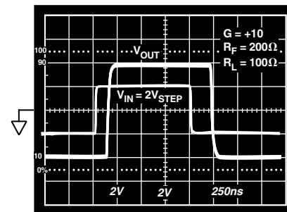
Figure 27. Overdrive Recovery; G = +10
