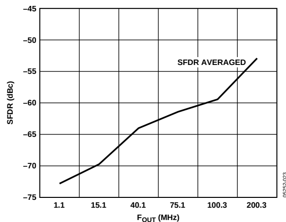
Figure 23. Averaged Channel SFDR vs. f_{OUT}
