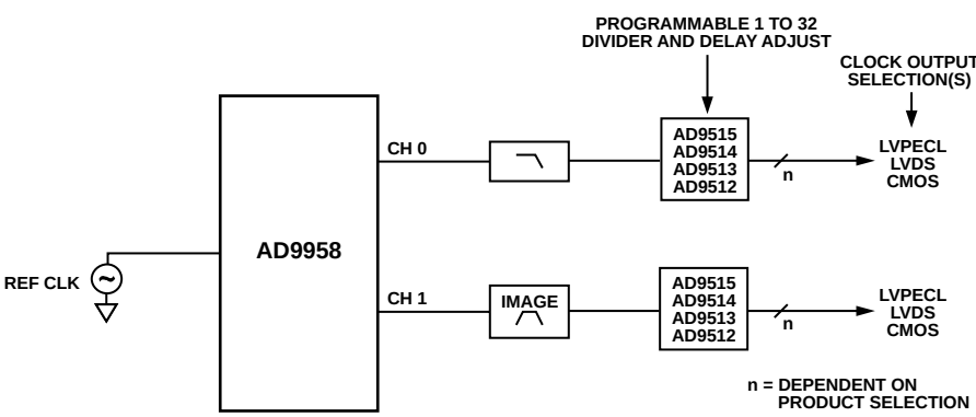
Figure 30. Clock Generation Circuit Using the AD951x Series of Clock Distribution Chips
