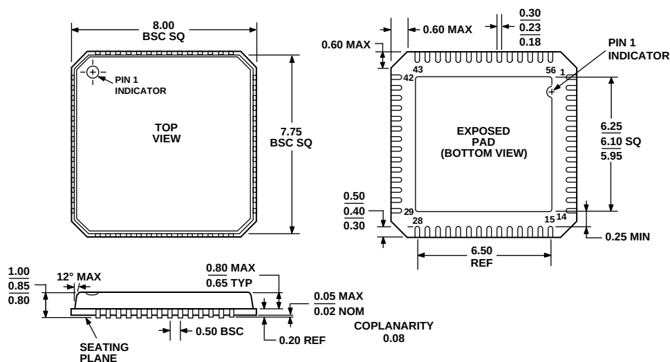
Figure 49. 56-Lead Lead Frame Chip Scale Package [LFCSP_VQ]
