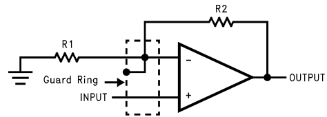
Non-Inverting Amplifier
