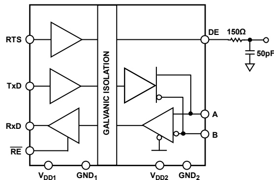
Figure 8. RTS-to-DE Propagation Delay
