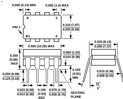
8-Lead Cerdip (Q-8)
