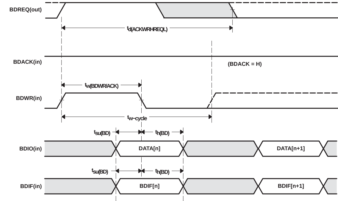
Figure 9–6. SCSI Burst Mode Write (4)
