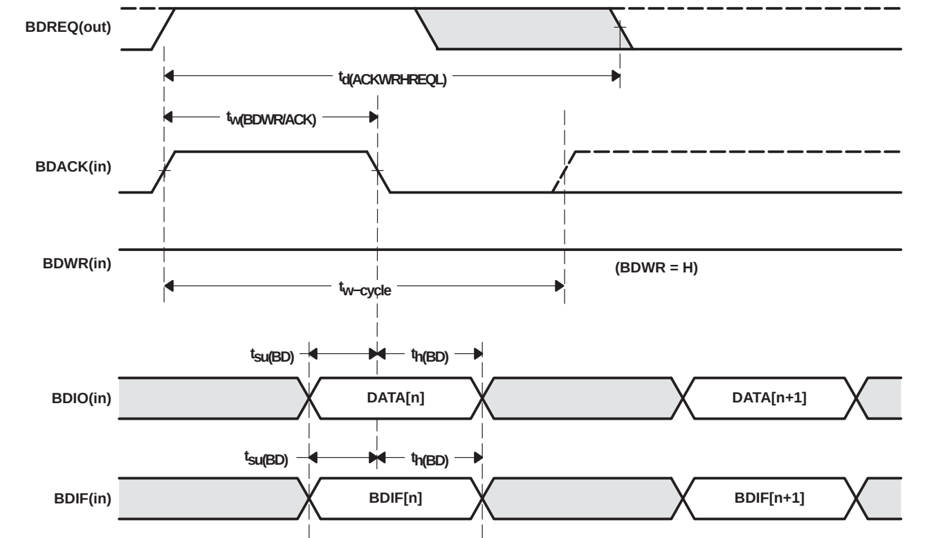
Figure 9–4. SCSI Burst Mode Write (2)
