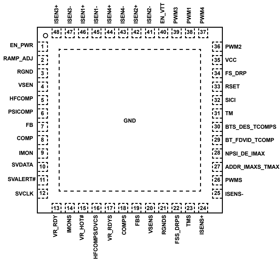
ISL6364 (48 LD 6X6 QFN) TOP VIEW
