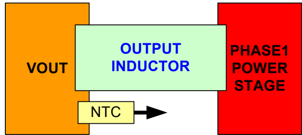
FIGURE 23. RECOMMENDED PLACEMENT OF NTC
