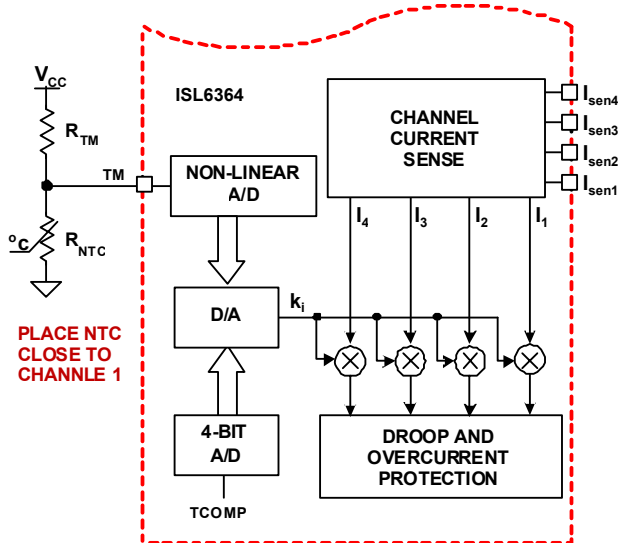
FIGURE 22. BLOCK DIAGRAM OF INTEGRATED TEMPERATURE COMPENSATION
