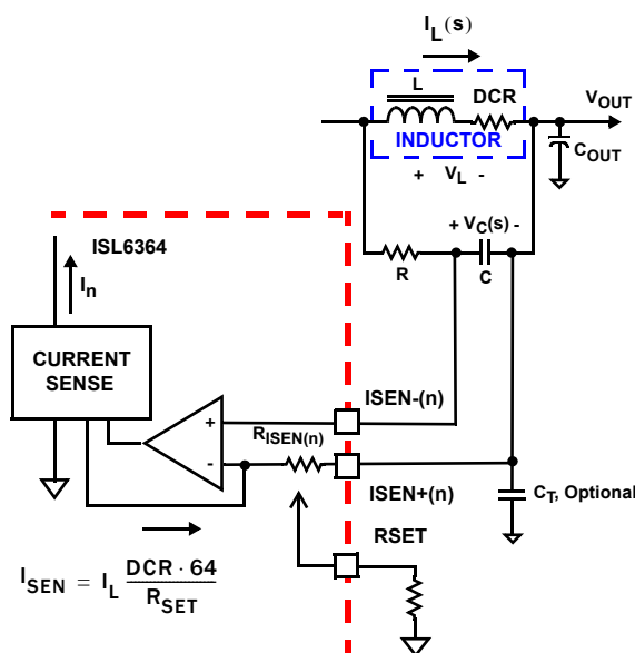
FIGURE 9. DCR SENSING CONFIGURATION FOR VR0
