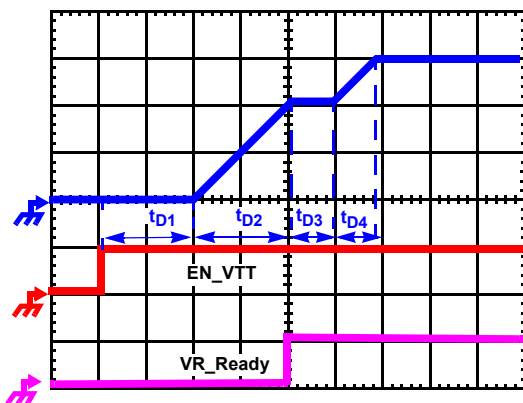
FIGURE 16. SOFT-START WAVEFORMS
