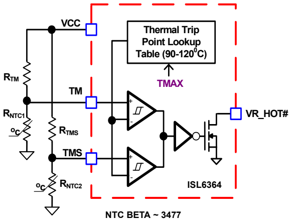
FIGURE 19. BLOCK DIAGRAM OF THERMAL MONITORING FUNCTION
