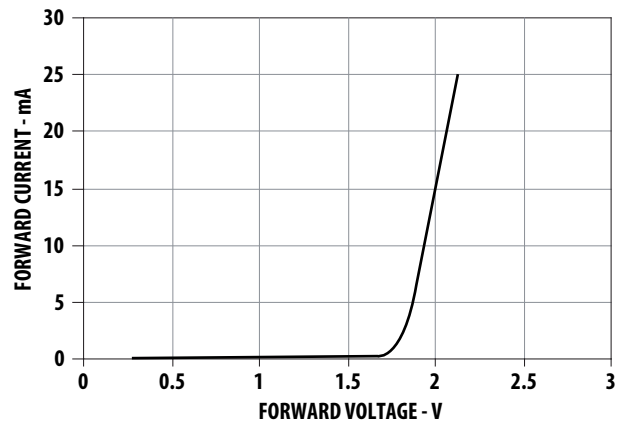
Figure 8. Forward Voltage Vs Current
