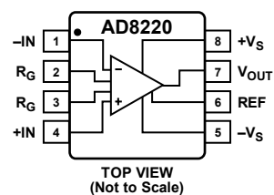
Figure 56. Pin Configuration
