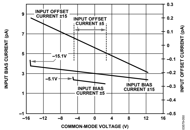
Figure 16. Input Current vs. Common-Mode Voltage
