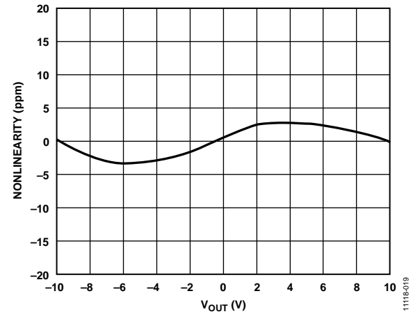
Figure 20. Gain Nonlinearity
