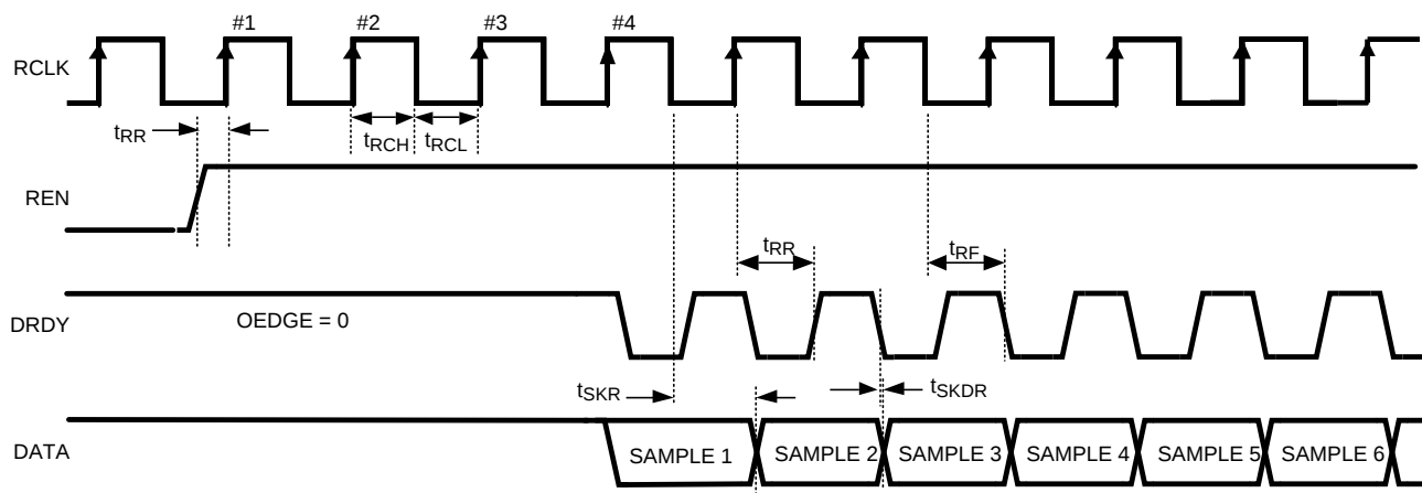
Figure 6. ADC08B200 Buffer Read Timing (OEDGE/TEN = 0)
