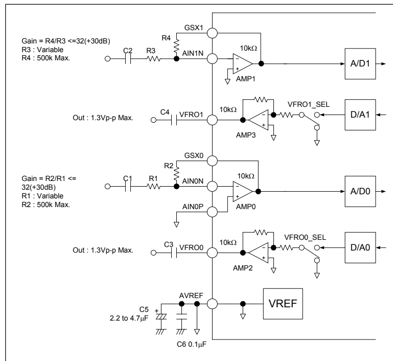
Figure 9 Analog Interface
