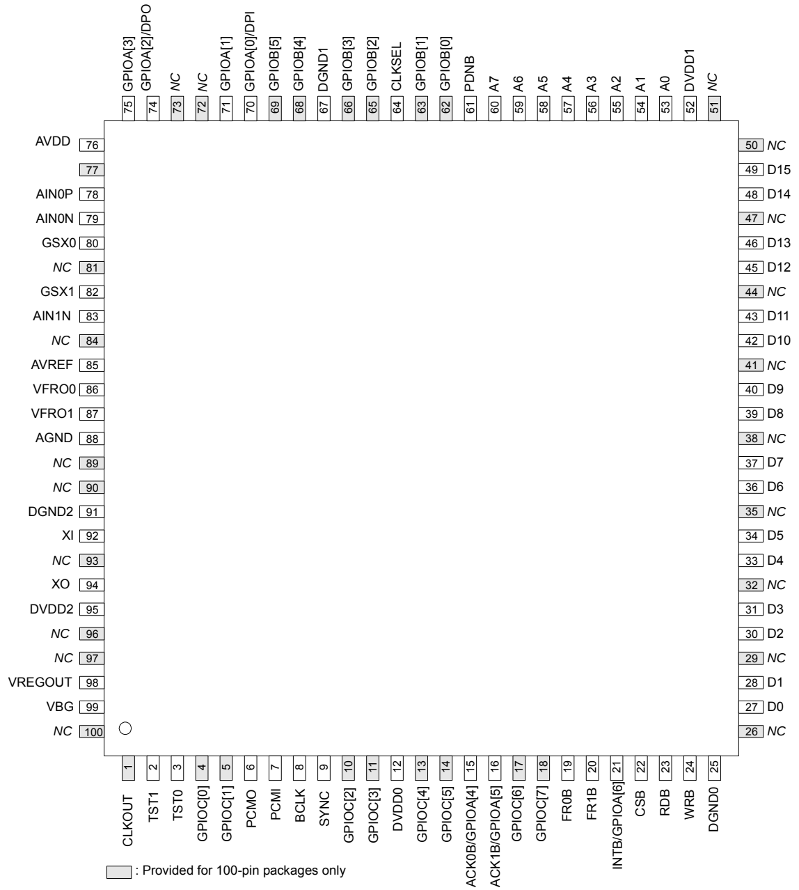
100-Pin Plastic TQFP
