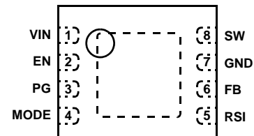
ISL9107 (8 LD 2X3 DFN) TOP VIEW
