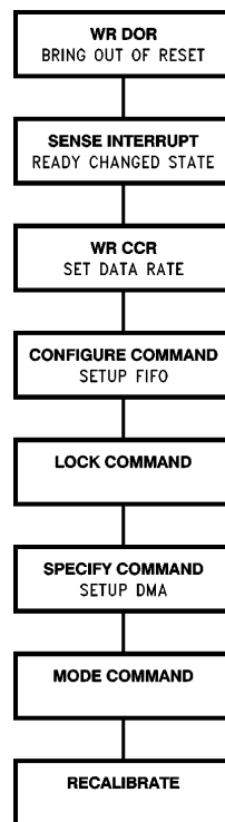
FIGURE 7-2. PC8477B Initialization
