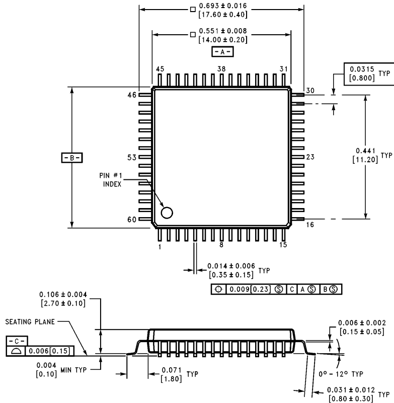
Plastic Quad Flat Package (PQFP) Order Number PC8477BVF-1 NS Package Number VF60A
