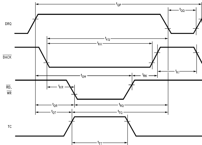
FIGURE 6-4. DMA Timing
