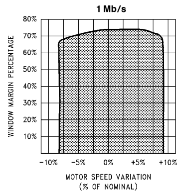
FIGURE 5-3. PC8477B Dynamic Window Margin Performance
