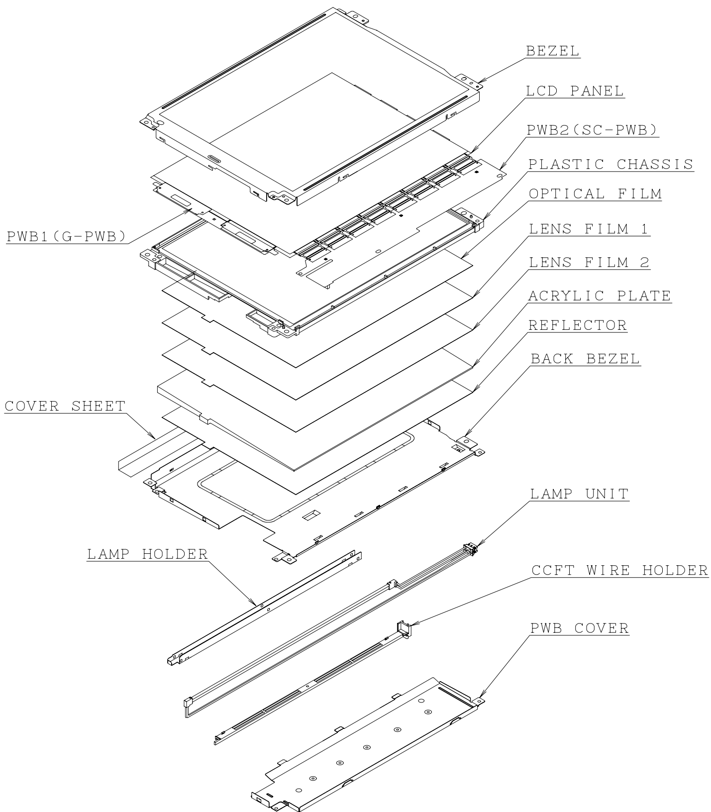
Fig4. Module Structure
