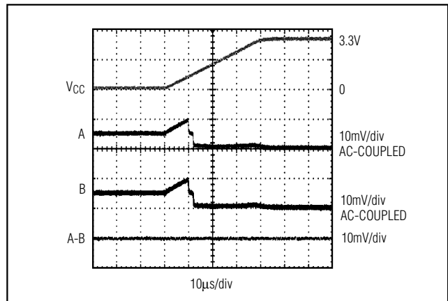
Figure 10. Differential Power-Up Glitch ( 0.1V/\mu s )
