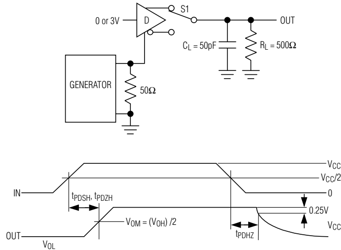
Figure 5. Driver Enable and Disable Times ( t_{PDSH} , t_{PDZH} , t_{PDHS} , t_{PDHZ} )
