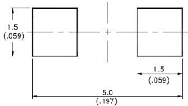
推荐焊盘尺寸 Recommended Soldering Pad
