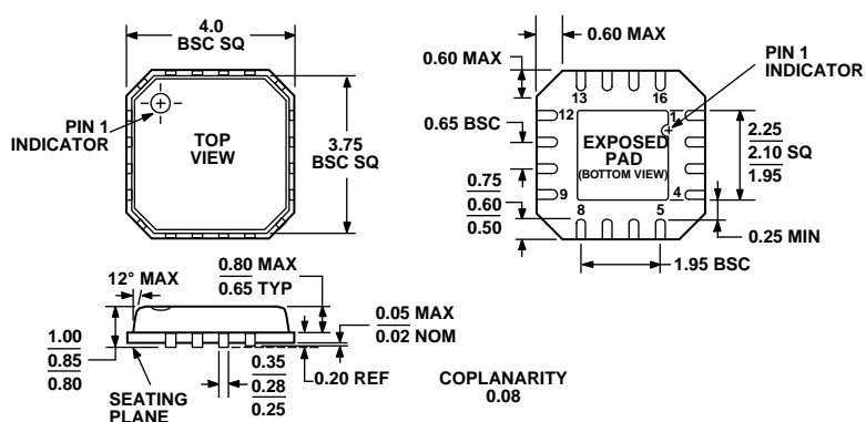
Figure 48. 16-Lead Lead Frame Chip Scale Package [LFCS] (CP-16)
